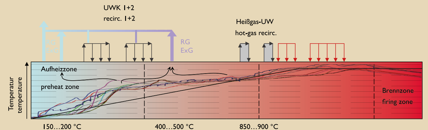
Prinzip LINGL PoroControl Principle LINGL PoroControl
